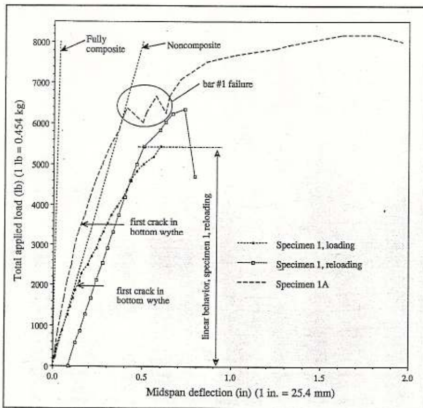
Fig. 6. Load-deflection curves for bending Specimens 1 and 1A.
