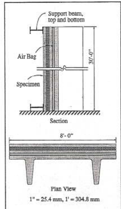
Fig. 10. Full scale flexural testing setup. (Connections of support beams to double tee not shown for clarity.)
