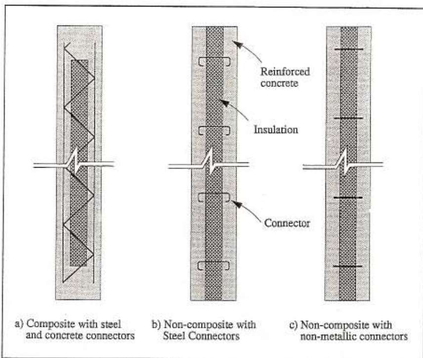
Fig. 1. Examples of existing PCSP systems.
