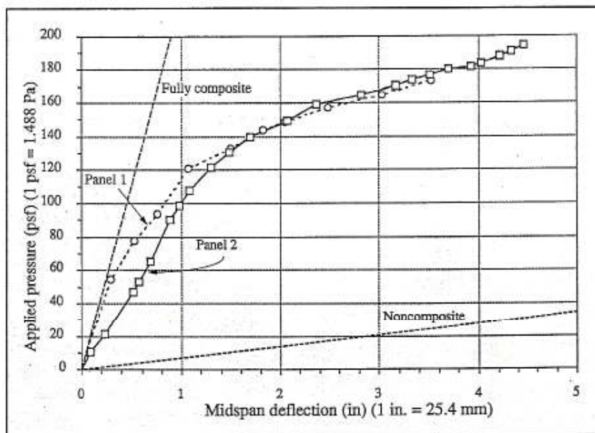
Fig. 11. Applied pressure vs. midspan displacement relationship.
