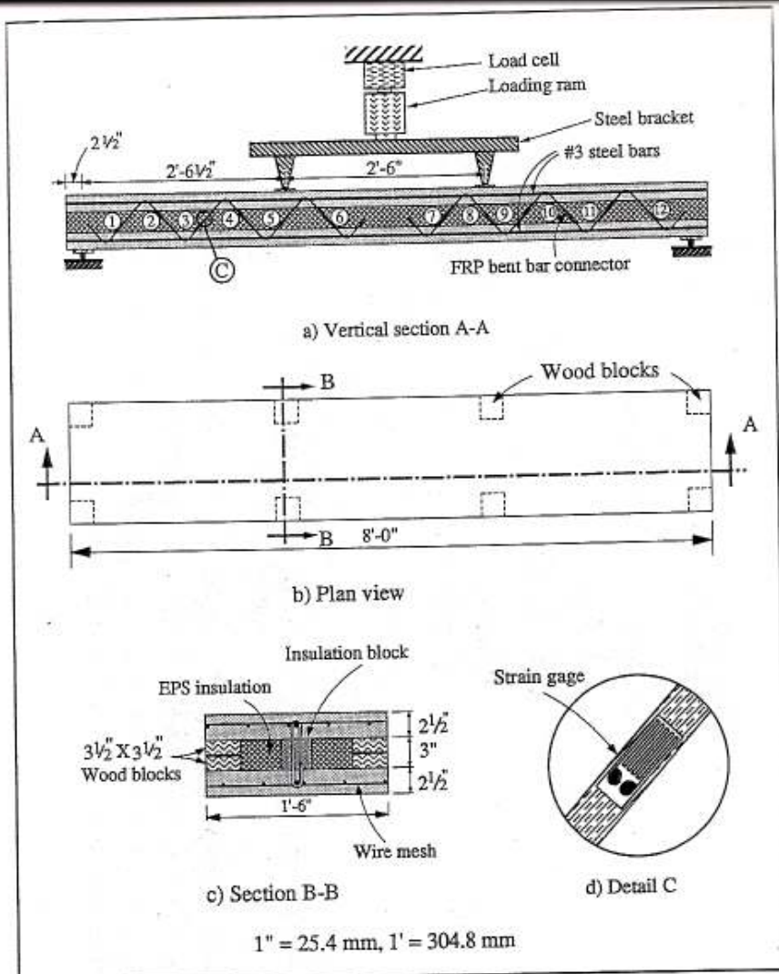
Fig. 5. Flexural test setup and details of specimens.
