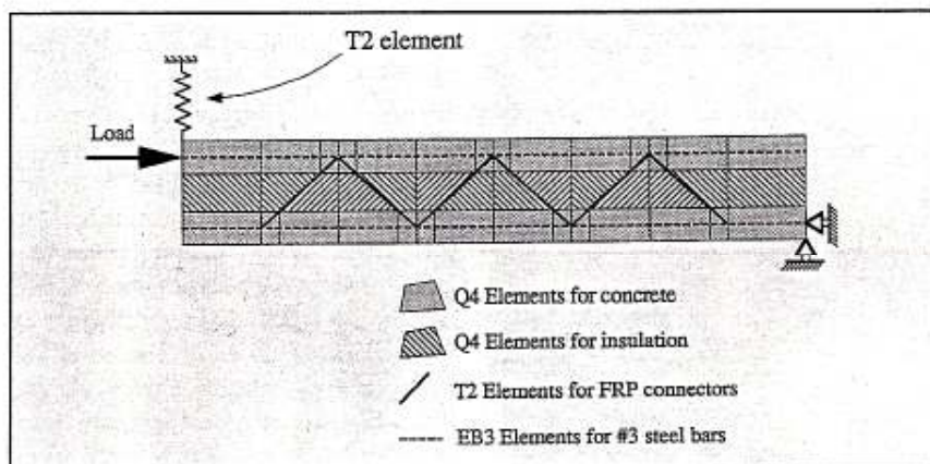
Fig. 12. Finite element model for shear specimens.
