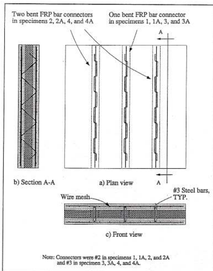
Fig. 4. Shear specimens.
