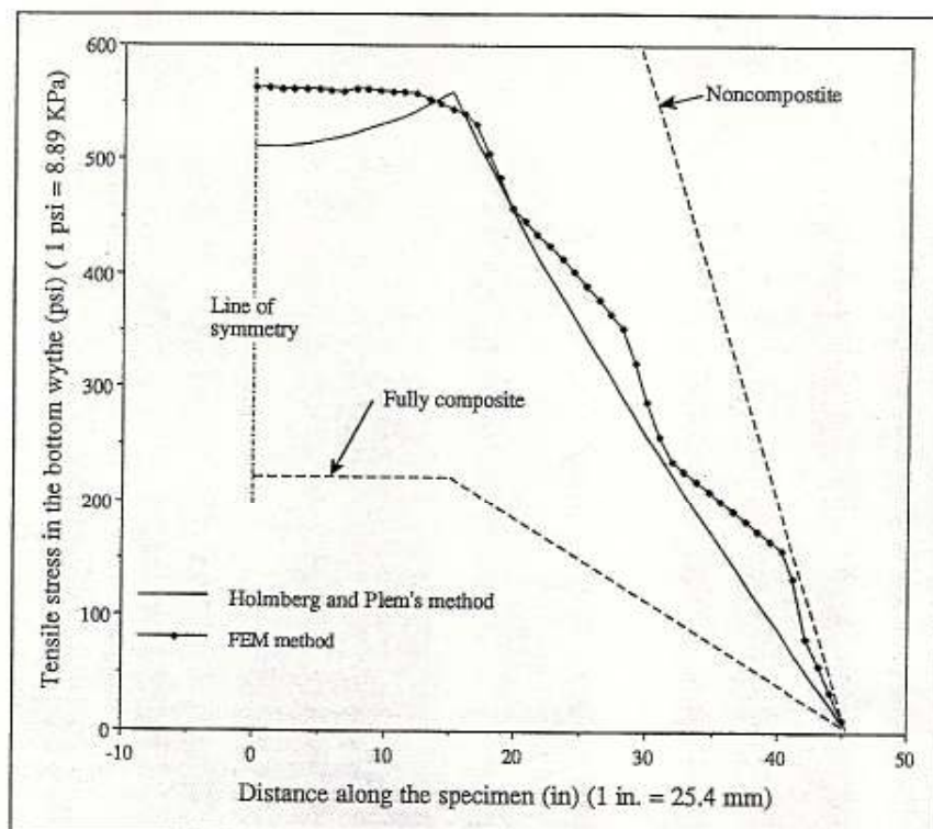
Fig. 17. Variation of maximum tensile stress in the bottom wythe of Specimen 1, at a total load of 2000 lbs (8.9 kN).
