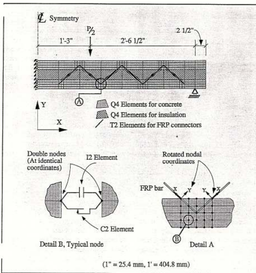
Fig. 14. Finite element model for small-scale flexural specimens.
