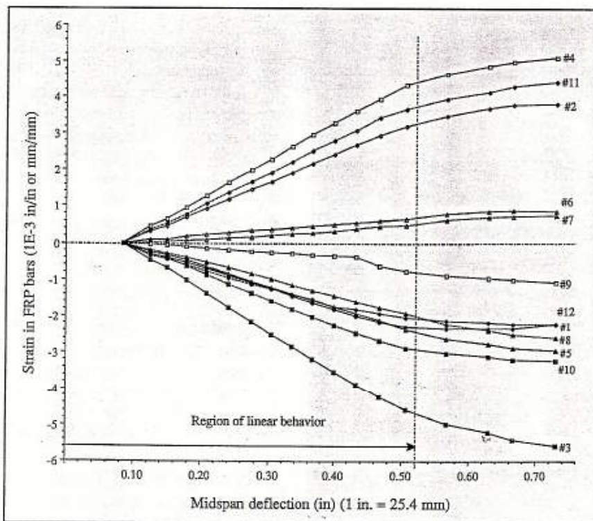
Fig. 7. Strain in FRP bars vs. midspan deflection for Specimen 1, reloading.
