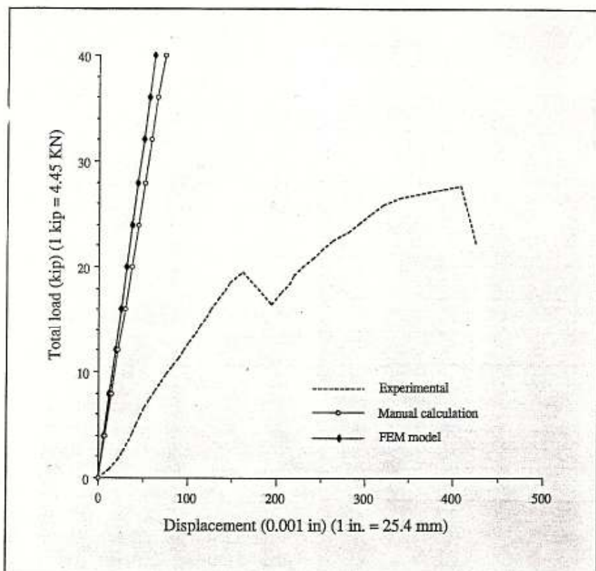
Fig. 13. Load-displacement curve for Shear Specimen 4.
