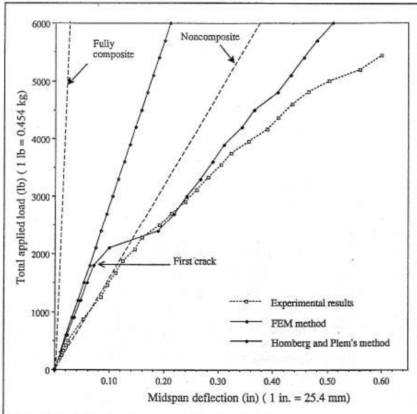
Fig. 15. Load-deflection curves for Specimen 1.
