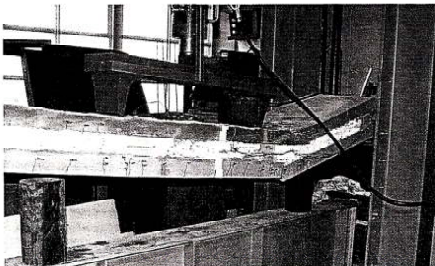
Fig. 9. Cracking pattern and failure of Specimen 1A.
